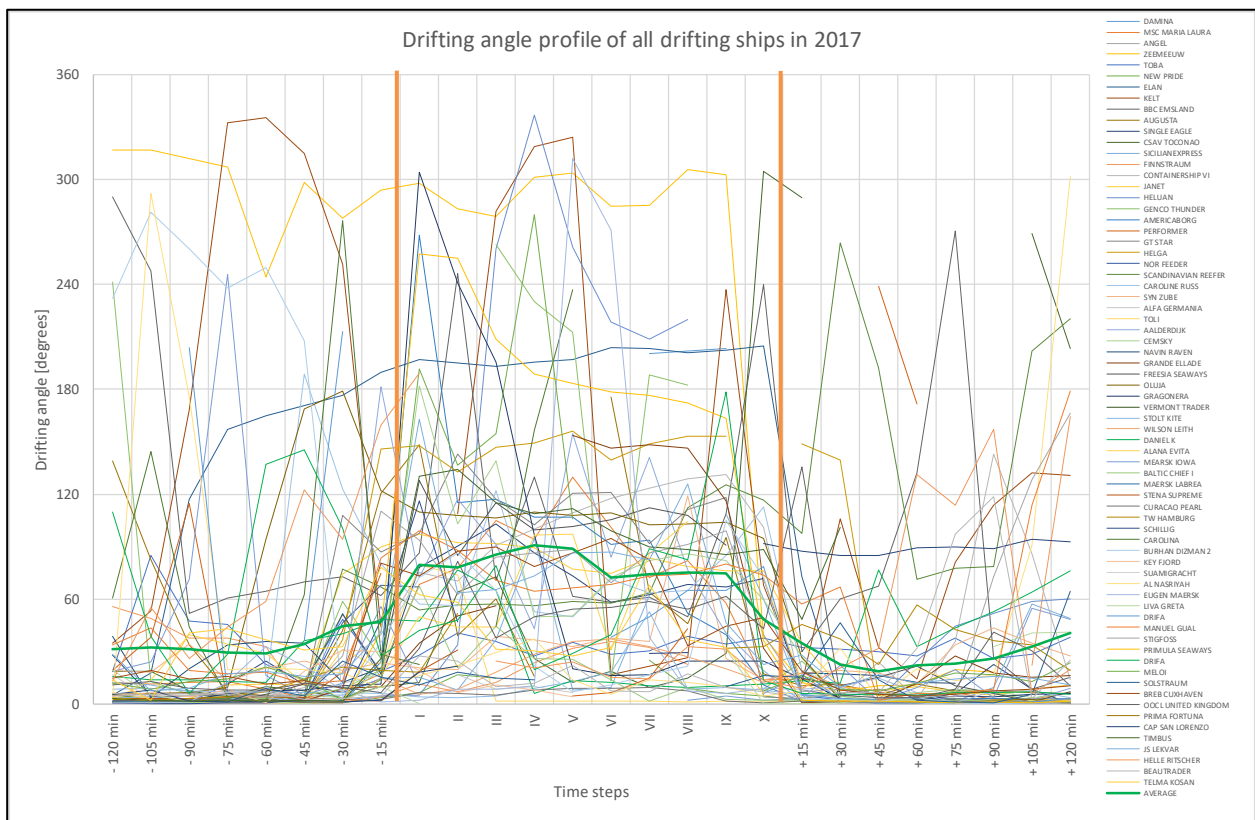
Figure 7-27 Average drift angle profile of all reported and analysed drifters in 2017
