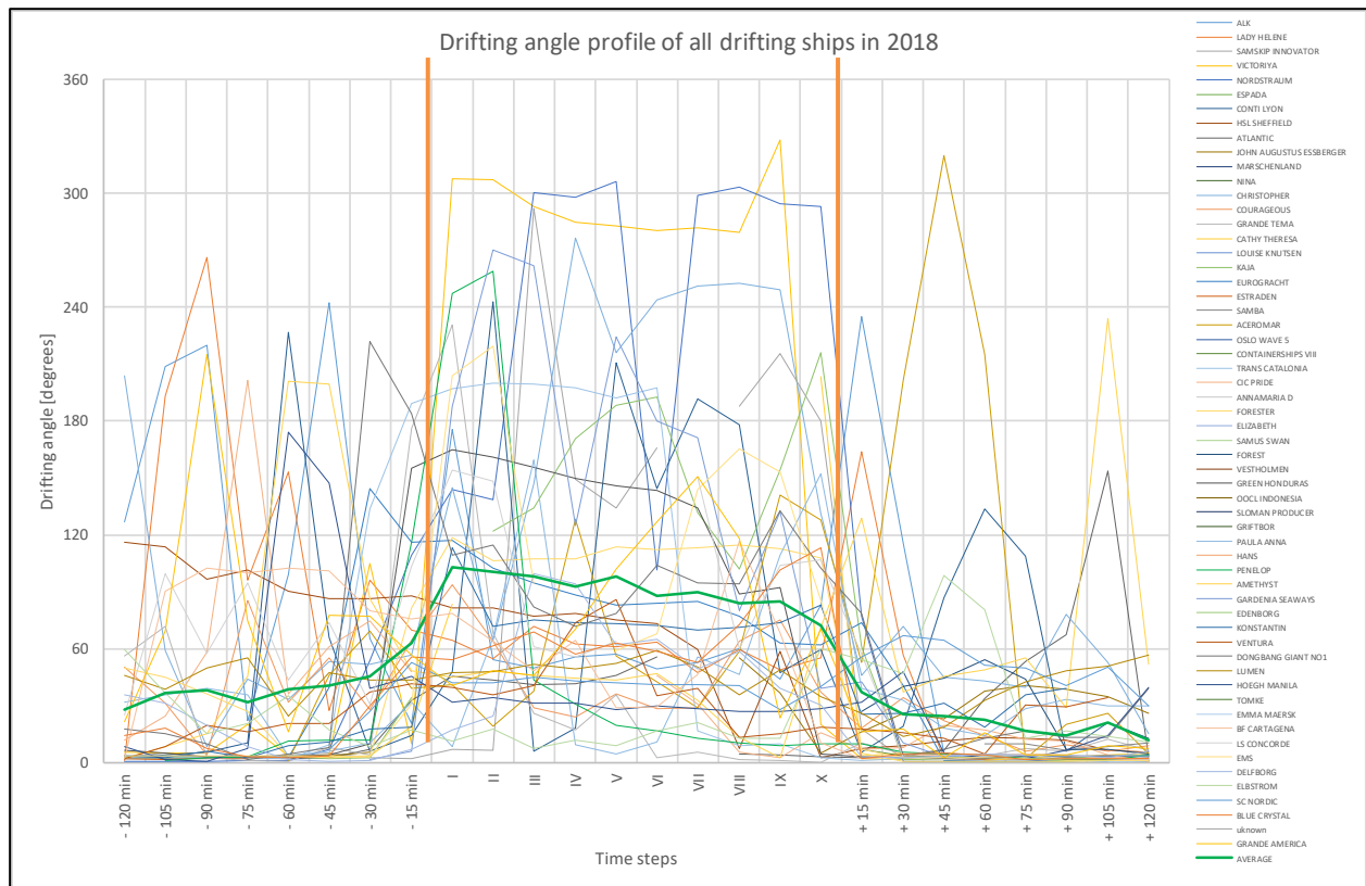
Figure 7-24 Average drift angle profile of all reported and analysed drifters in 2018
