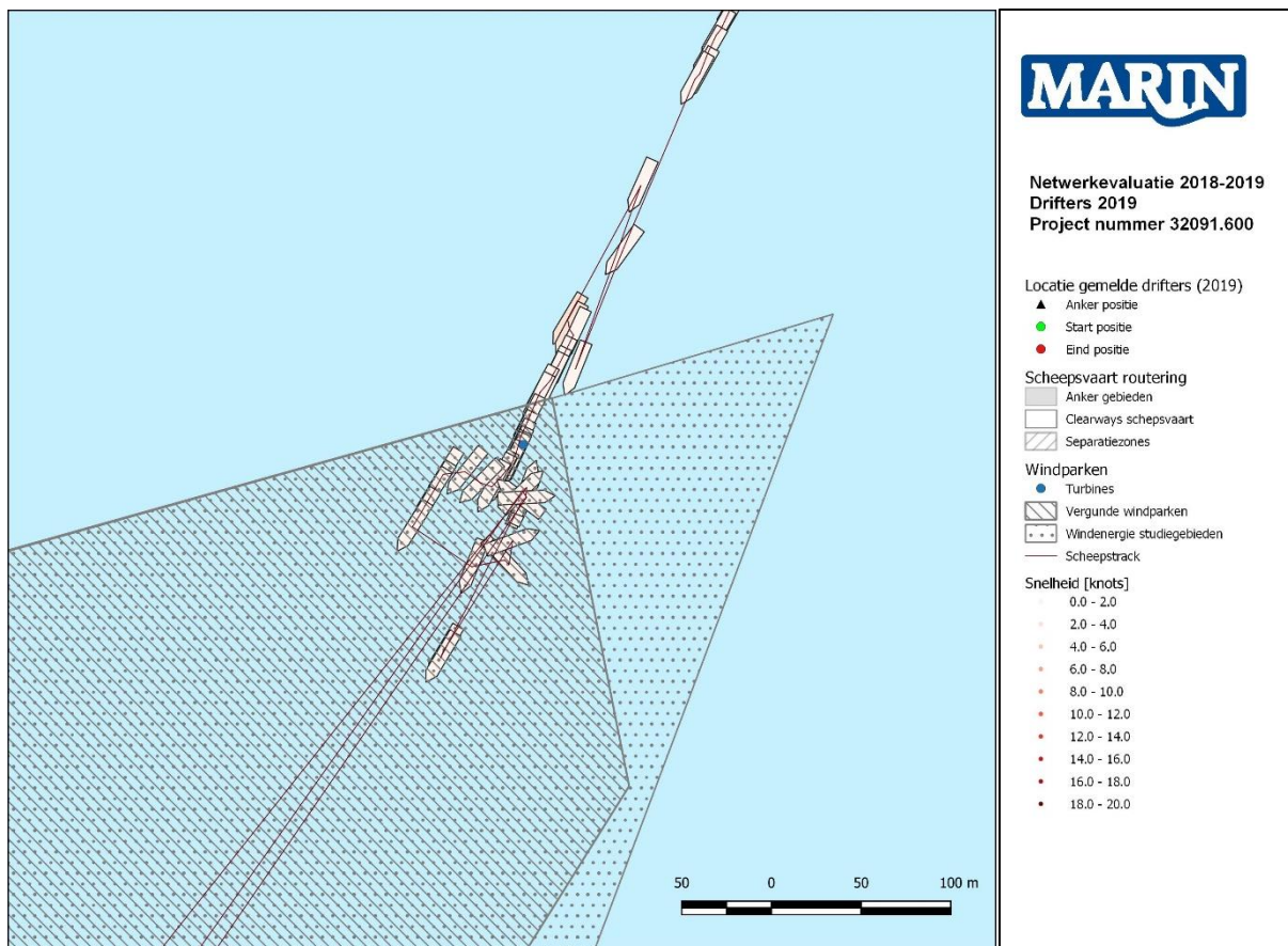
Figure 7-9 Ship collision with OWT Luchterduinen Cargo vessel (90m)
