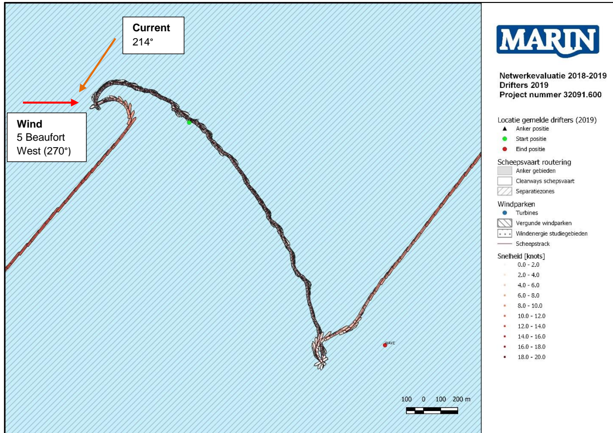
Figure 7-14 Environmental impact during drifting and ship contour of cargo vessel
