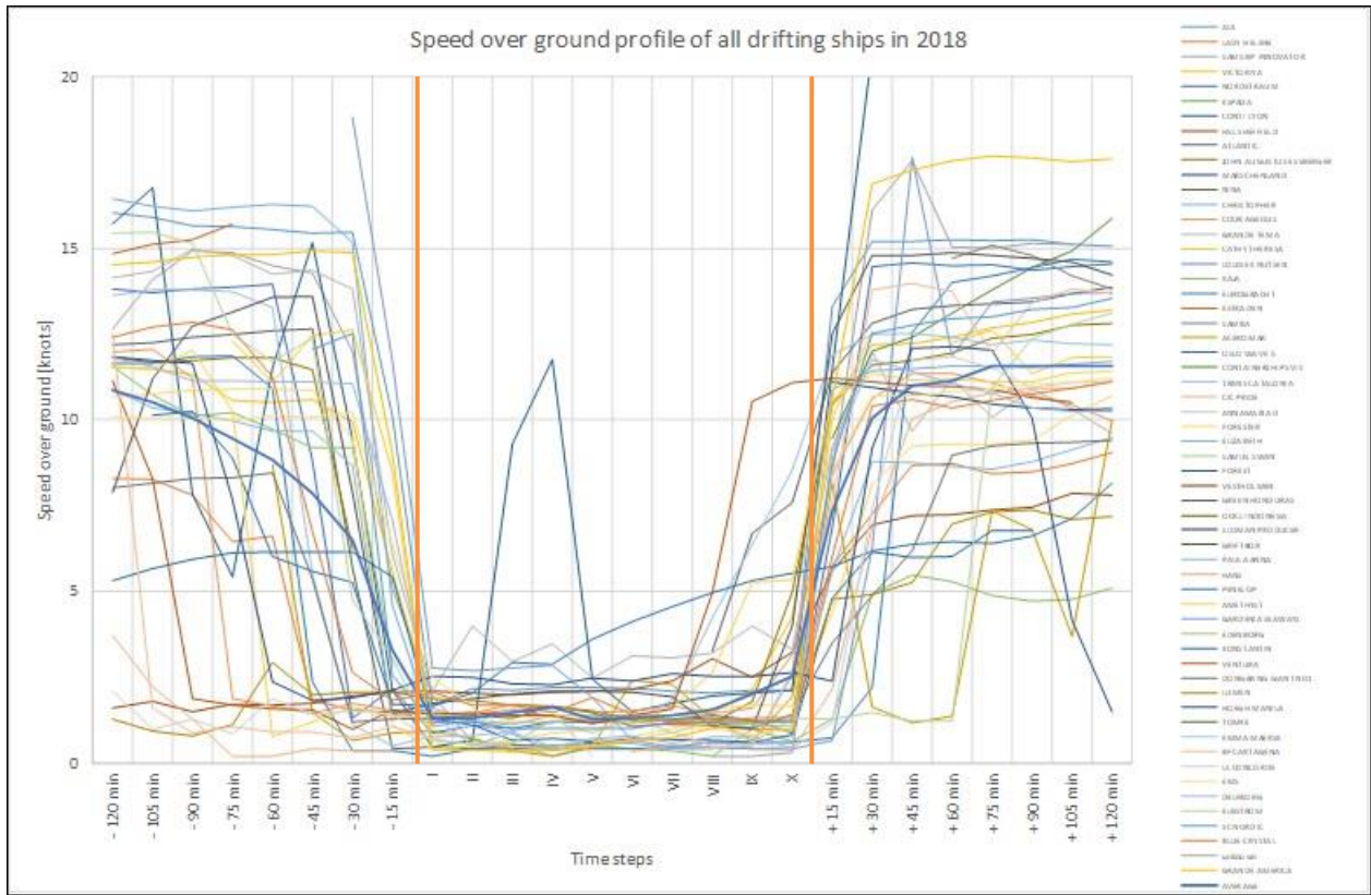
Figure 7-23 Average speed profile for all reported and analysed drifters in 2018
