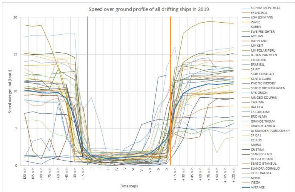
Figure 7-20 Average speed profile for all reported and analysed drifters in 2019
