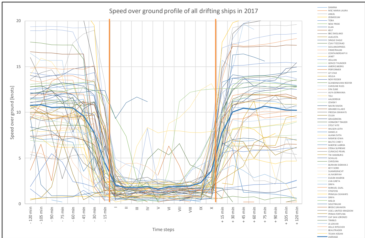
Figure 7-26 Average speed profile for all reported and analysed drifters in 2017
