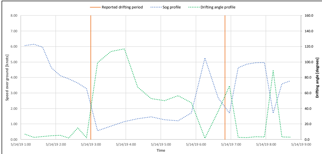
Figure 7-5 Average speed and drift angle profile of Standby Guard Vessel
