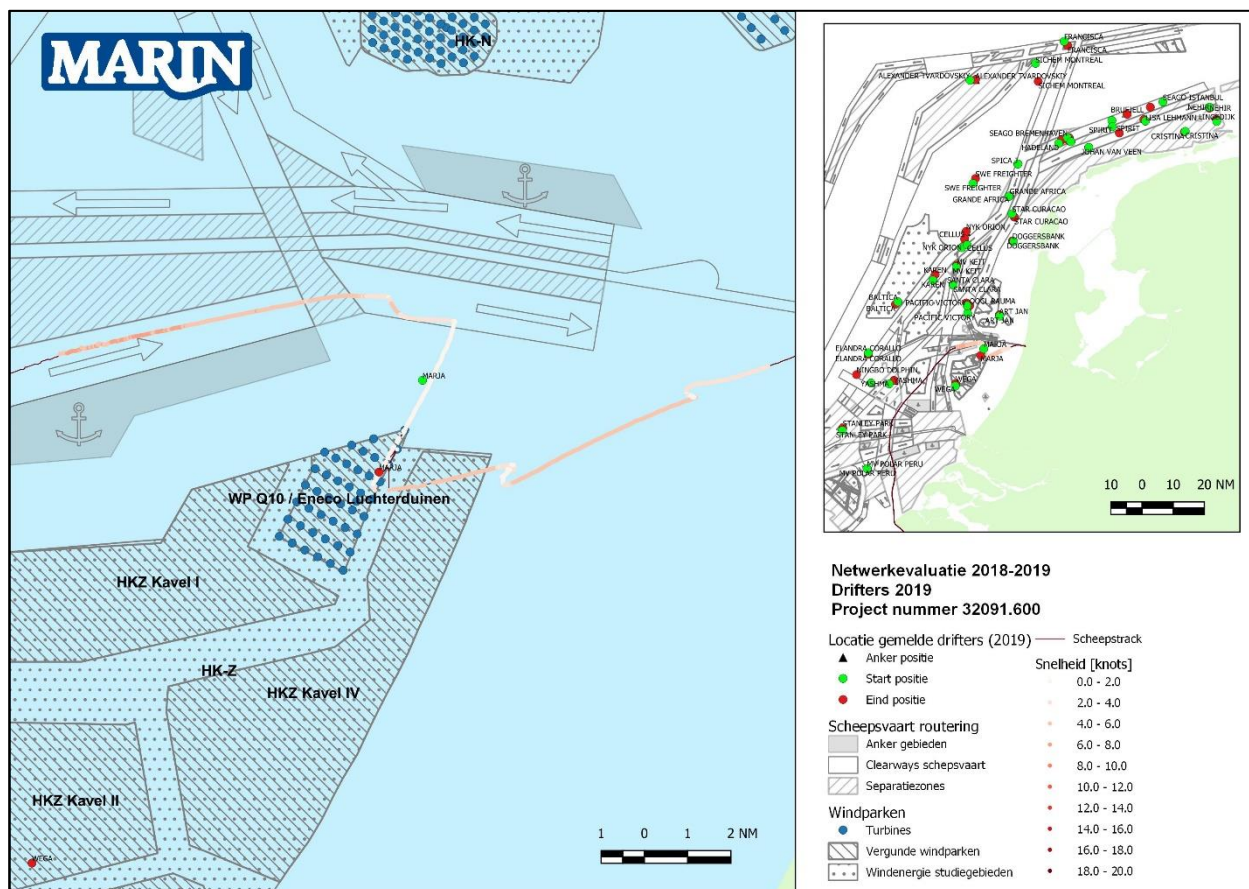
Figure 7-2 Drifting of Standby Guard Vessel
