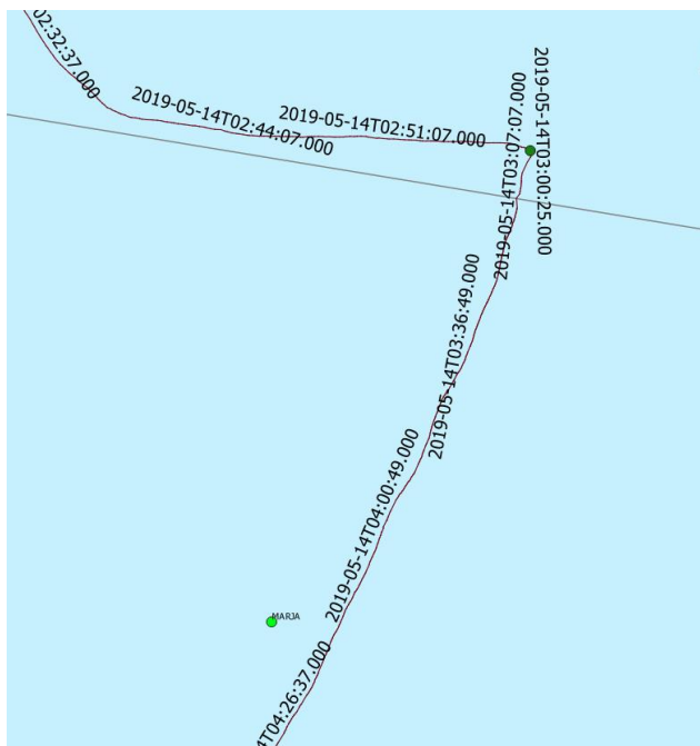
Figure 7-30 Example of position inaccuracy
