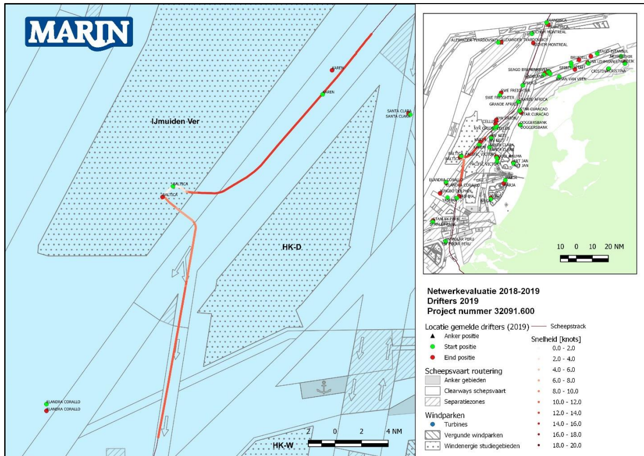
Figure 7-15 Drifting cargo vessel (158m)
