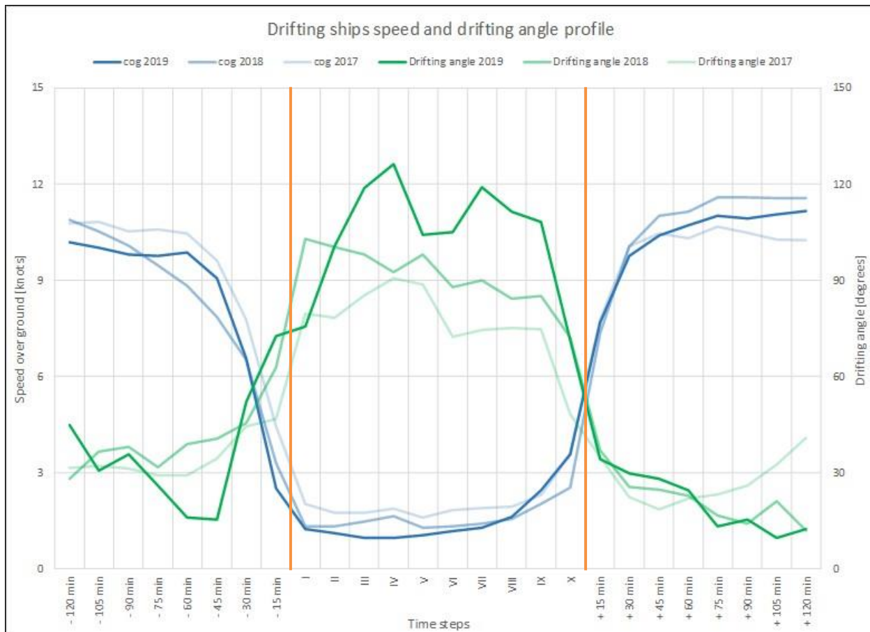
Figure 7-29 Average speed and drift angle profile per time steps in 2017-2019
