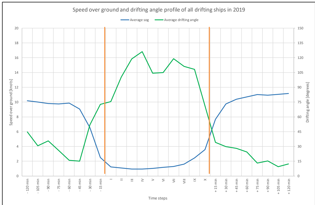
Figure 7-22 Average speed and drift angle profile per time steps in 2019
