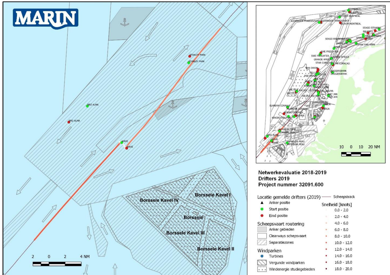
Figure 7-10 Drifting cargo vessel
