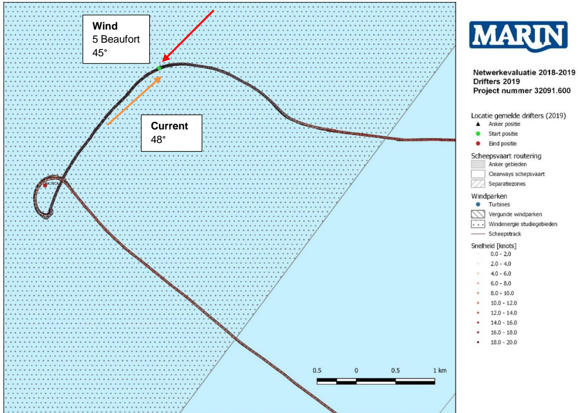
Figure 7-19 Environmental impact during drifting and ship contour of cargo vessel (158m)
