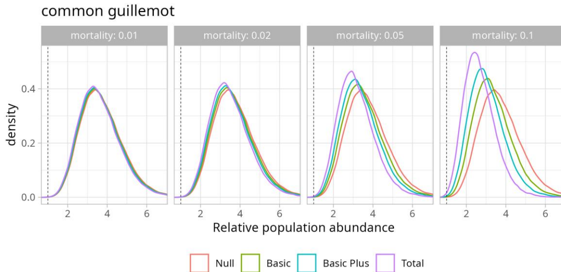
Figure 4-18 Probability distributions of population abundances after 40 simulated years, relative to the initial mean population abundance, for the common guillemot and the national OWF scenarios. Different panels show different mortality probabilities used in calculating the mortality effect of displacement. The distributions for the Null scenario are identical between panels. Each distribution is scaled such that mean initial population abundance equals 1 (vertical dashed line).
