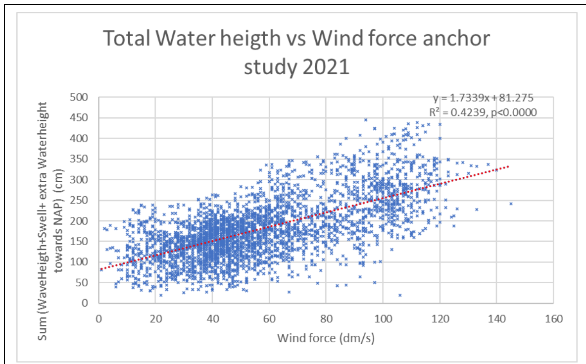
Figure 5 Relation between the Indicator Haul-out (Equation 1, Sum (Wave Heigth+Swell+extra Water Height towards NAP) (cm)) and wind force for 2021 (data from Rozemeijer et al., 2021b).
