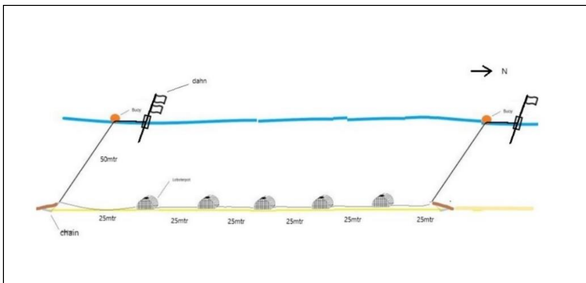
Figure 1 Crab-pot-strings with five pots and two chains. Next to the buoy a dahn is attached (buoy with flag(s), counterweight and radar reflector). The double flag indicates the most southern buoy of the string. A single flag indicates the most northern buoy. In this set up mutual distance between the pots is 25m but 40m is used as well for statistical reasons (Skerrit, 2014).
