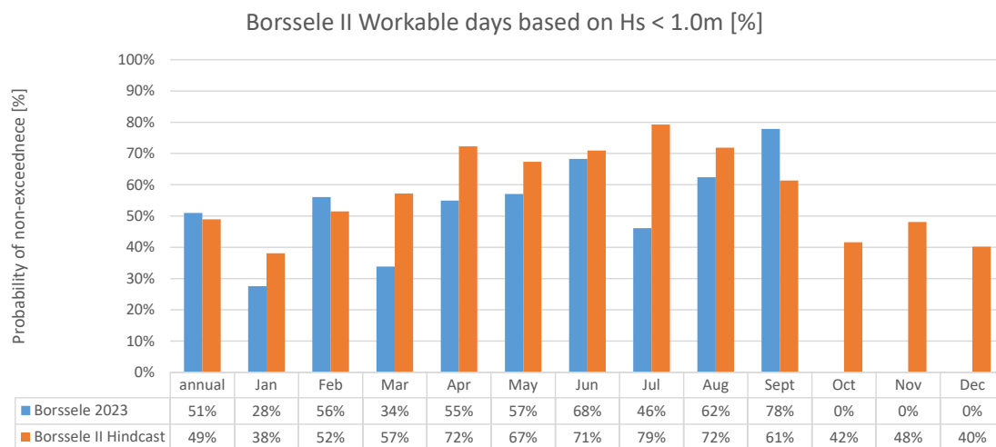
Figure 3.2.5 - Workable days based on wave height criteria H_s < 1.0\text{m} in Borssele 2023 (blue) and average (blue).
