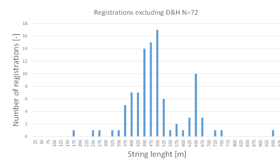
Figure 3.3.1 - Calculated string lengths between first and second anchor during setting excluding D & H.
