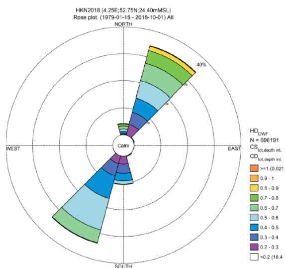
Depth-integrated current roses (going to) at HKN2018: total current (source: Metocean Study; HK(N)WFZ (2019), Figure 8.41)
