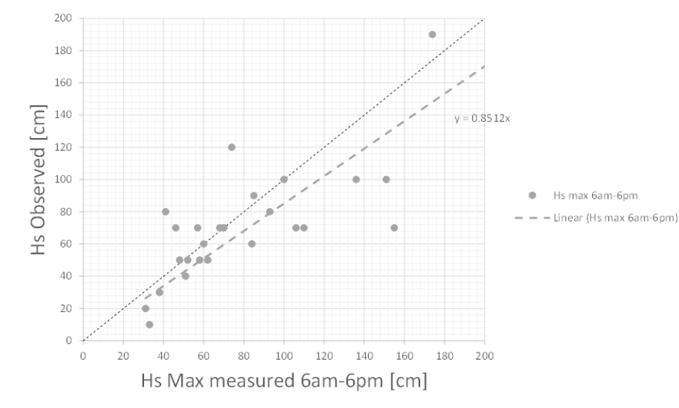
Figure 3.2.1 - Observed wave height versus measured maximum wave height during daytime on sailing days.
