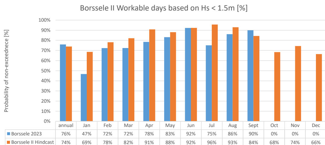
Figure 3.2.6 - Workable days based on wave height criteria H_s < 1.5\text{m} in Borssele 2023 (blue) and average (blue).
