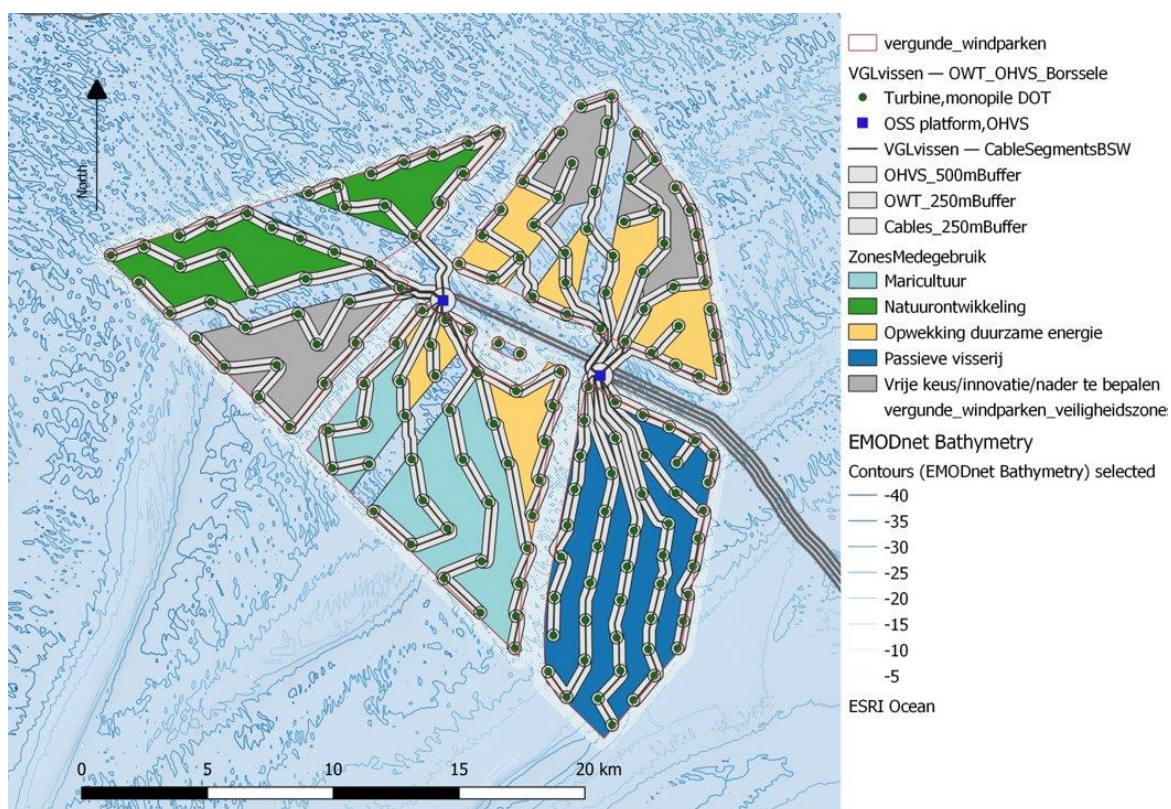
Figure 2.4.5 - Locations of Borssele I and II offshore wind farm. For the gill net and multi-species pot experiments plot II (blue area) was used. For handline and jigging experiments both plot I (grey area in the North) and II (blue area in the South) were used except for the fishery free zone, as indicated in Figure 2.1.1.
