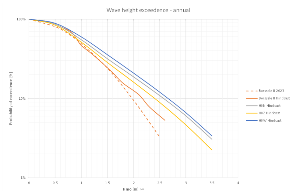
Figure 3.4.1 - Annual probability of wave height exceedance
