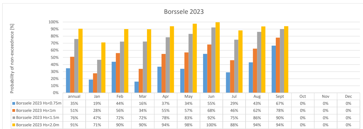
Figure 3.4.2 - Monthly workable days in Borsselle 2023 (measured; probability of non-exceedance)
