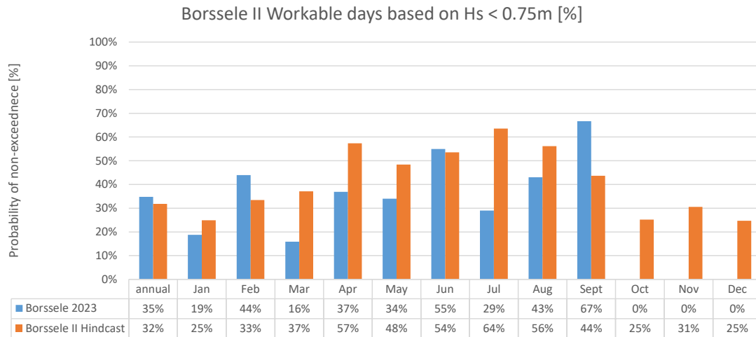
Figure 3.2.4 - Workable days based on wave height criteria H_s < 0.75\text{m} in Borssele 2023 (blue) and average (blue).
