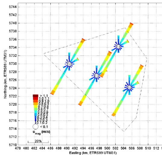
Annual current roses in the BWFZ (source: Deltares, 2015, Figure 6.2)
